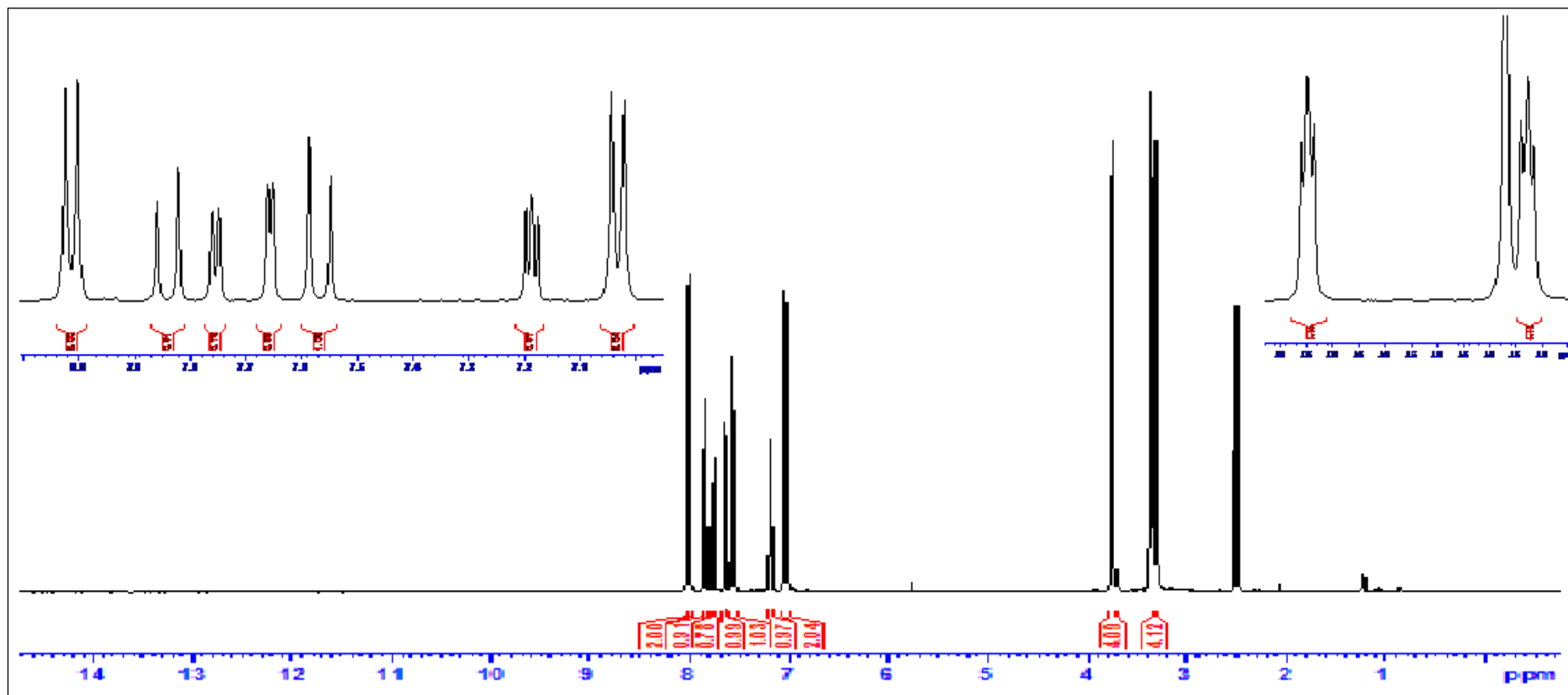
Figure 5. ^1\text{H} NMR spectrum of compound 2
