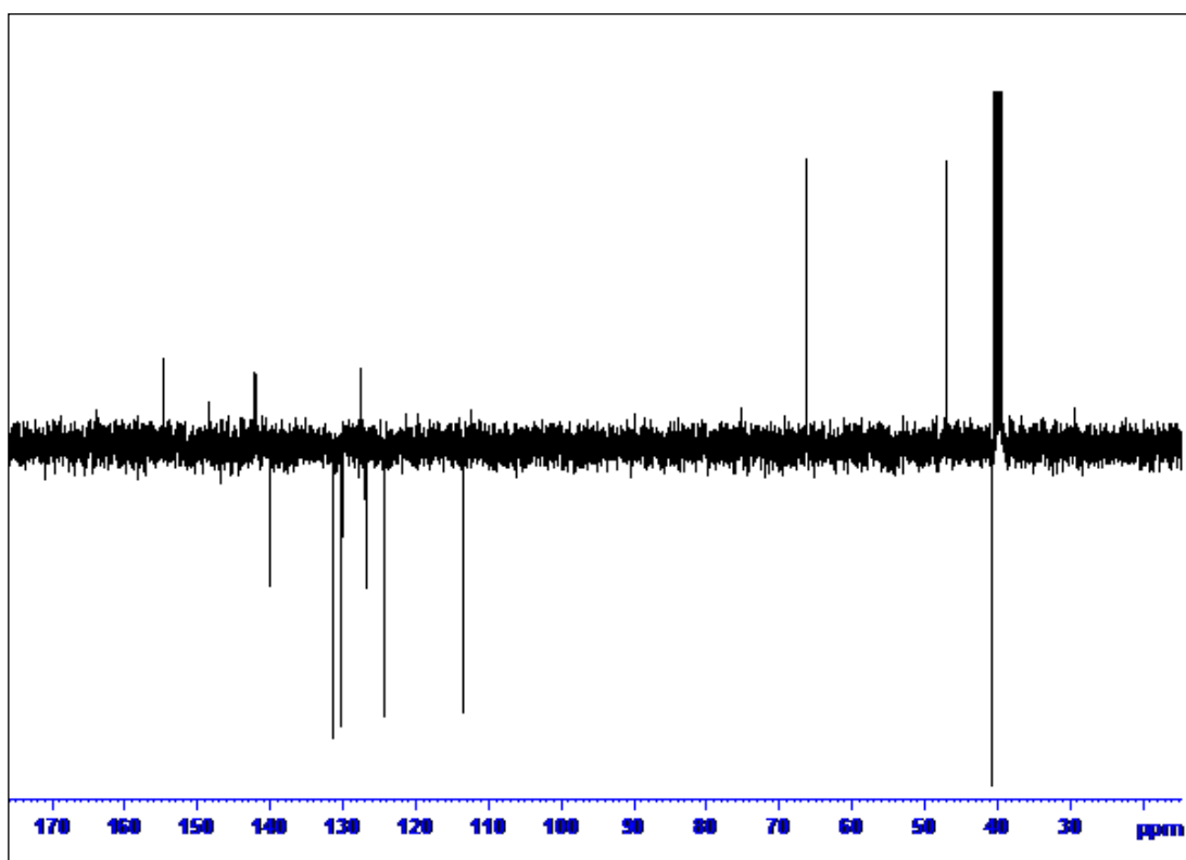
Figure 33. APT spectrum of compound 10
