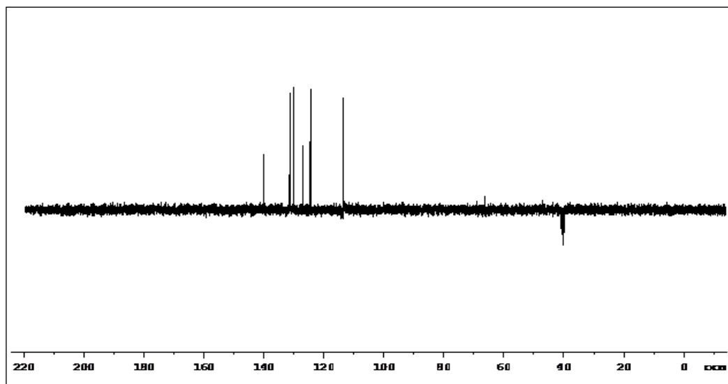
Figure 32. DEPT 90 spectrum of compound 10
