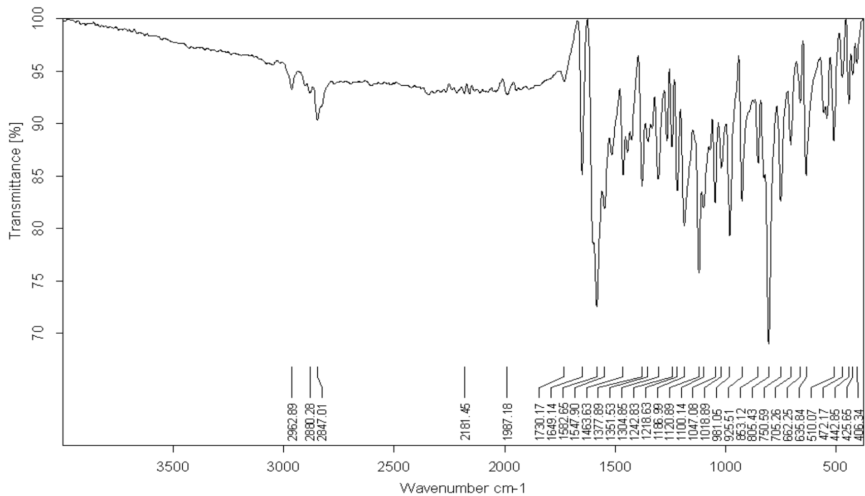
Figure 13. FT-IR spectrum of compound 5
