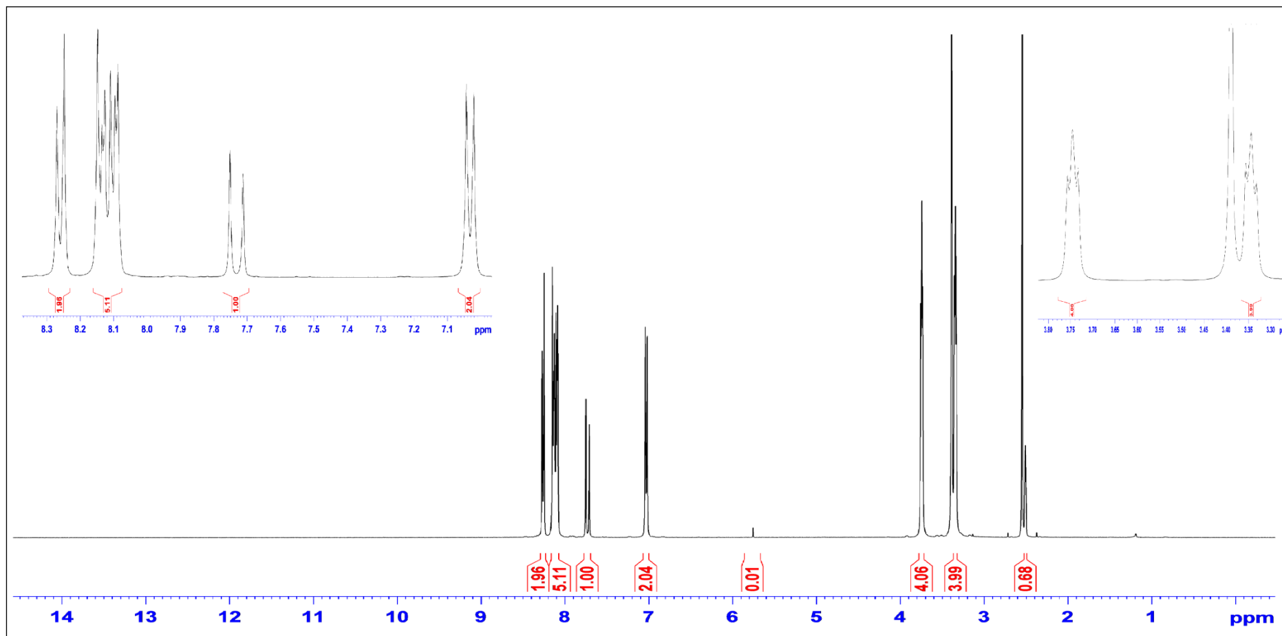
Figure 30. ^1\text{H} NMR spectrum of compound 10
