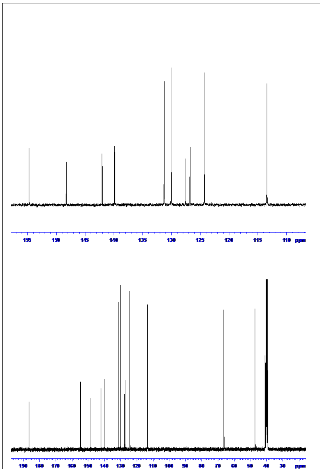
Figure 31. ^{13}\text{C} NMR spectrum of compound 10
