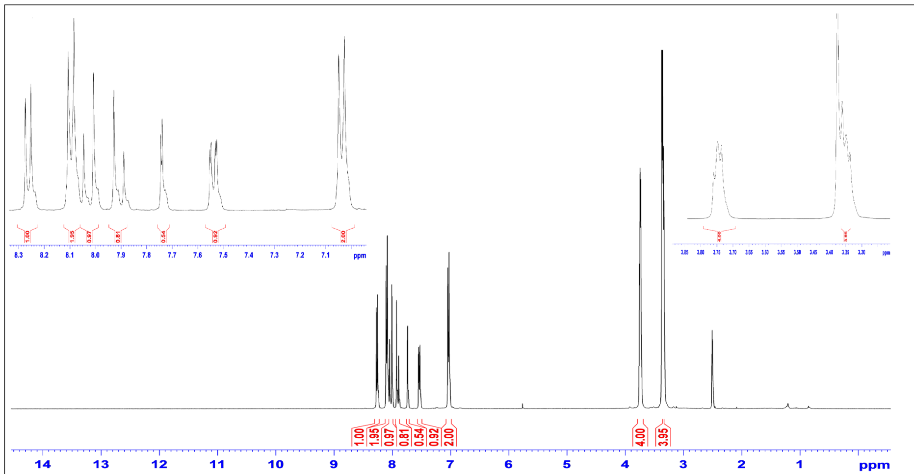
Figure 14. 1 H NMR spectrum of compound 5
