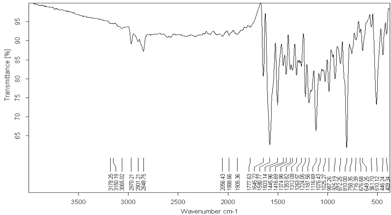
Figure 18. FT-IR spectrum of compound 7
