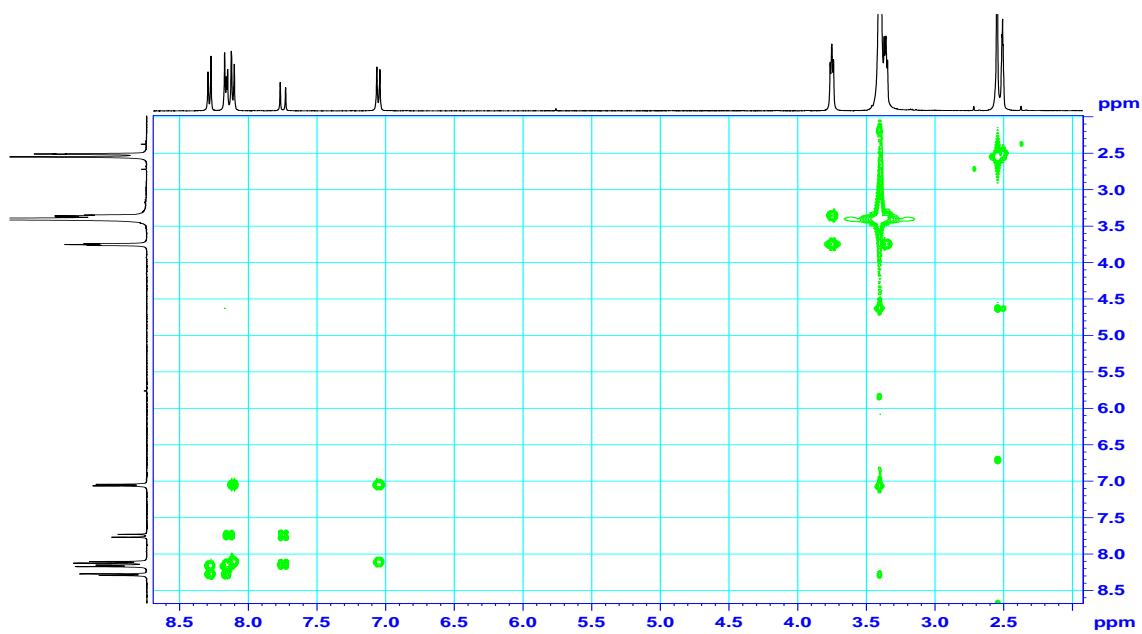
Figure 35. HETCOR spectrum of compound 10
