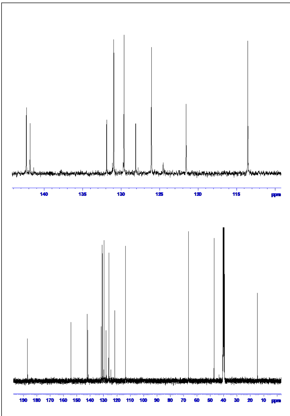
Figure 23. ^{13}\text{C} NMR spectrum of compound 8
