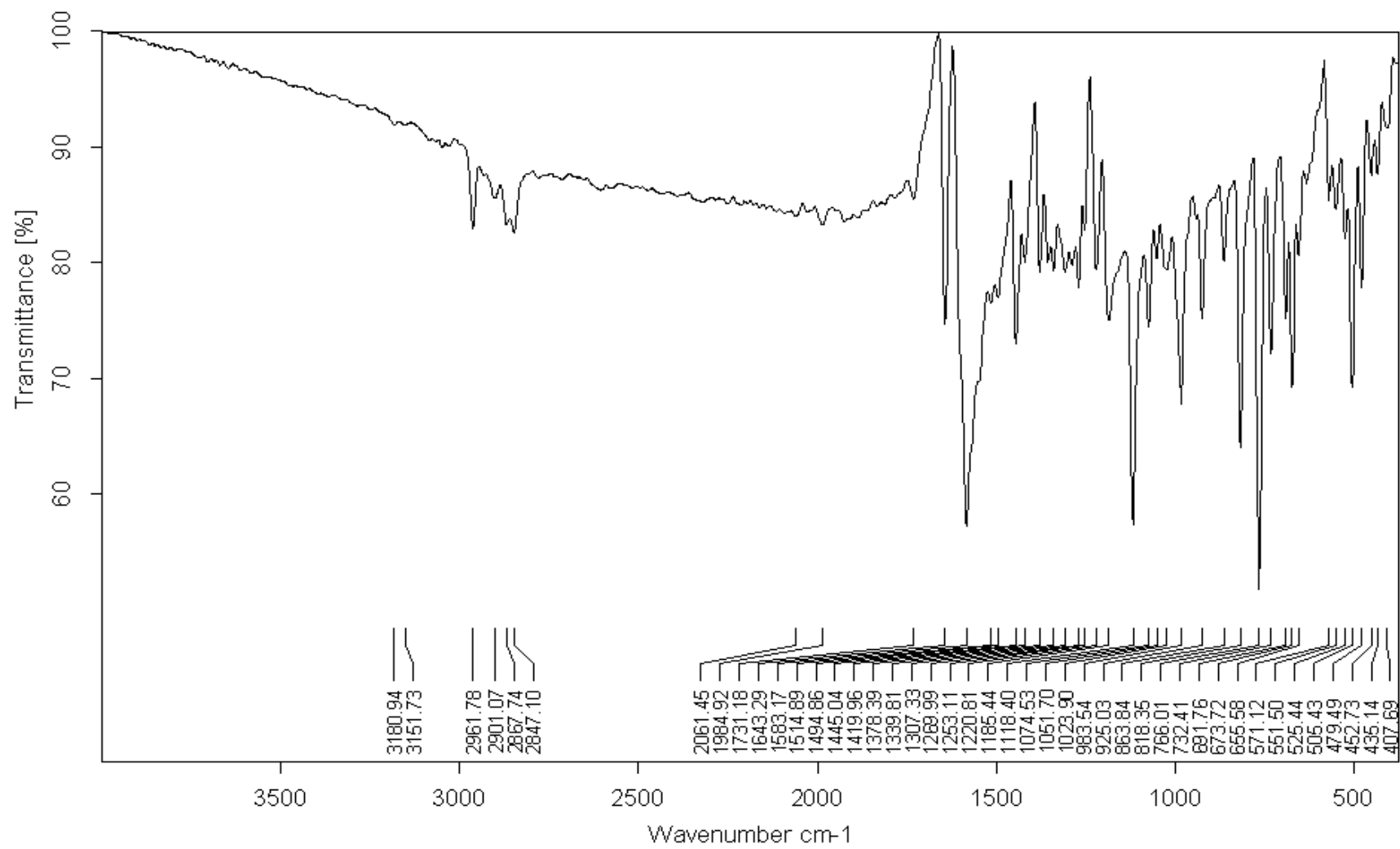
Figure 7. FT-IR spectrum of compound 3
