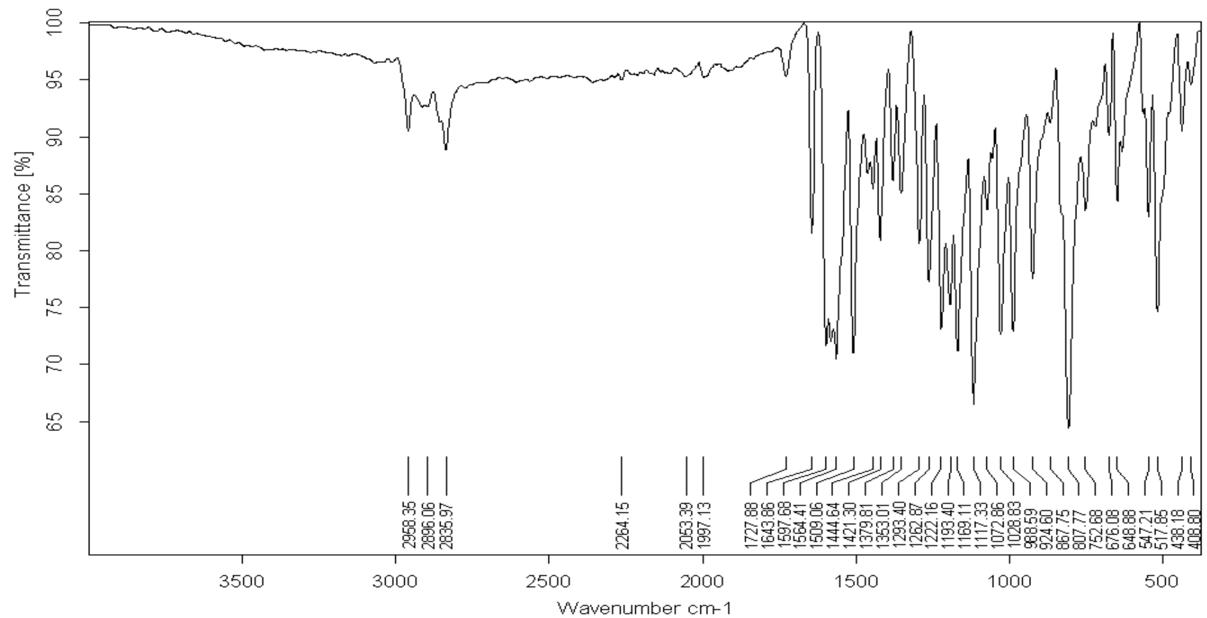
Figure 26. FT-IR spectrum of compound 9
