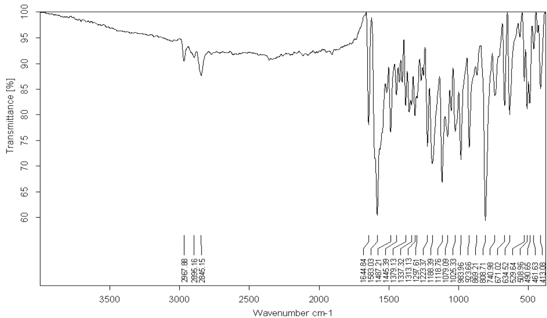
Figure 10. FT-IR spectrum of compound 4
