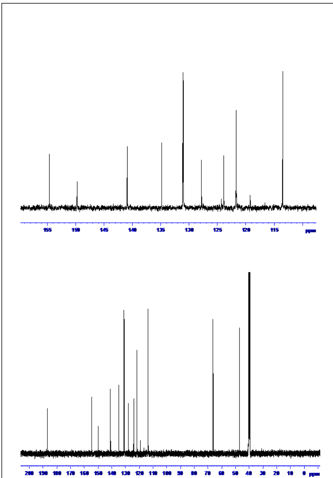
Figure 28. ^{13}\text{C} NMR spectrum of compound 9
