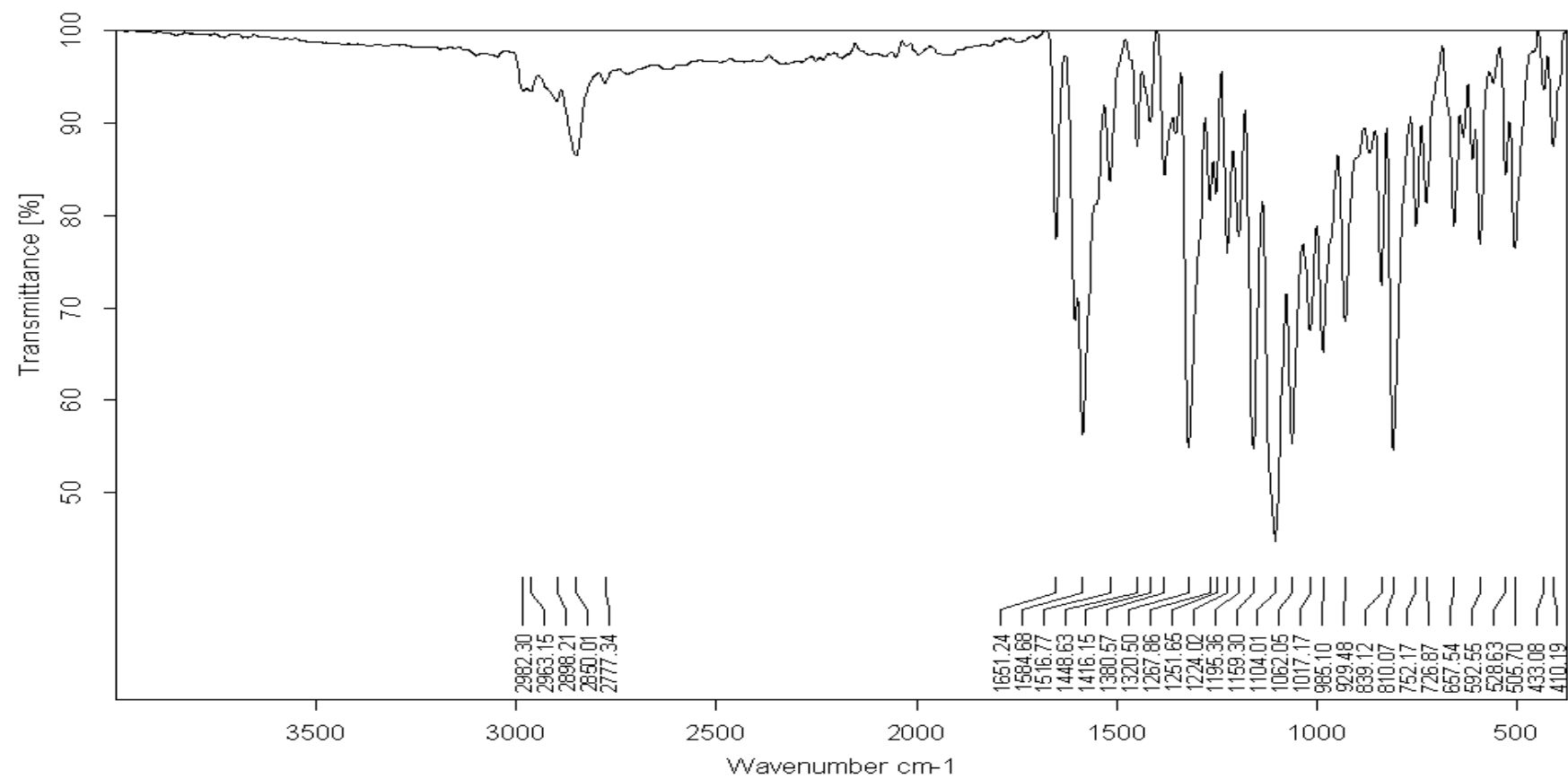
Figure 37. FT-IR spectrum of compound 11
