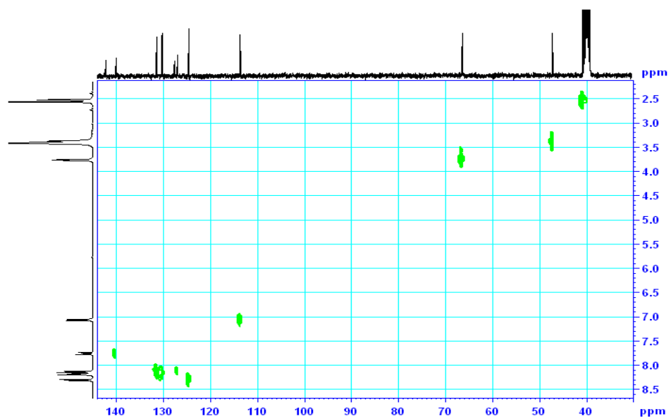
Figure 34. COSY spectrum of compound 10
