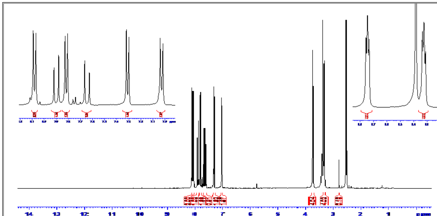
Figure 24. 1 H NMR spectrum of compound 8
