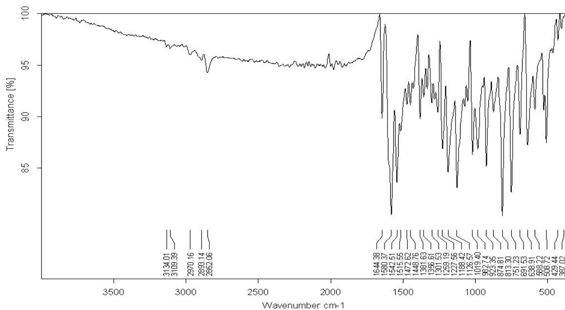
Figure 1. FT-IR spectrum of compound 1
