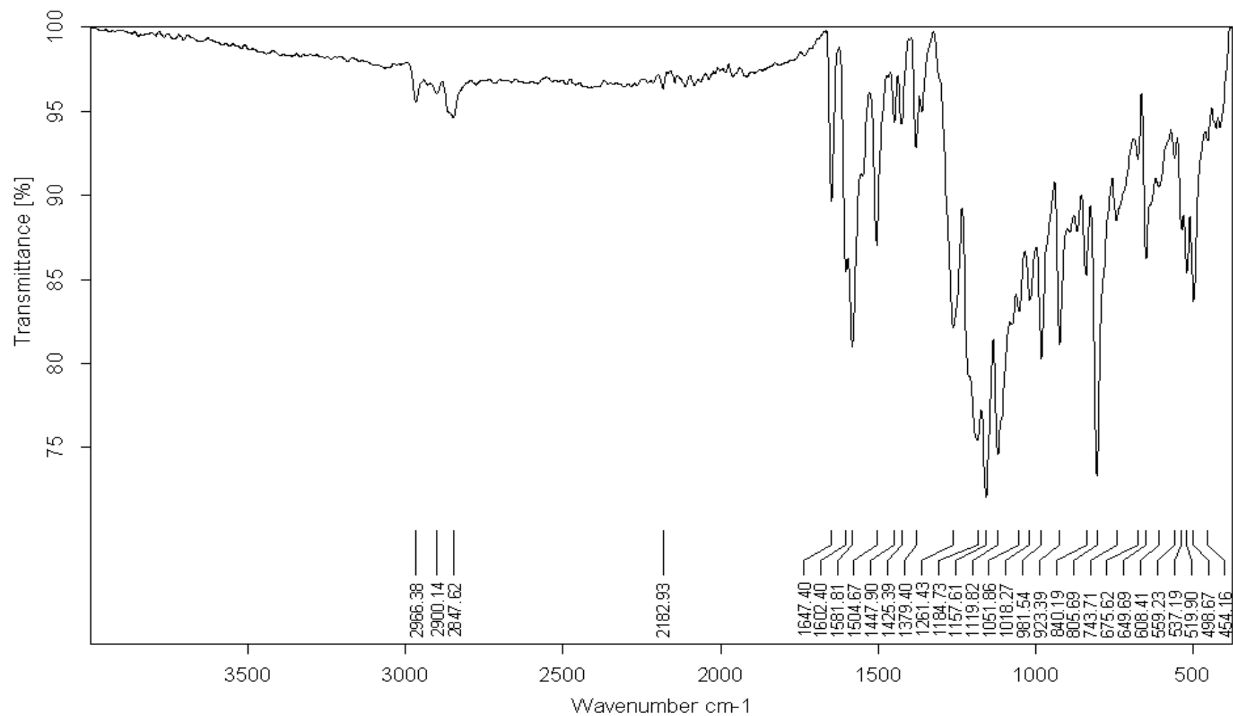
Figure 40. FT-IR spectrum of compound 12
