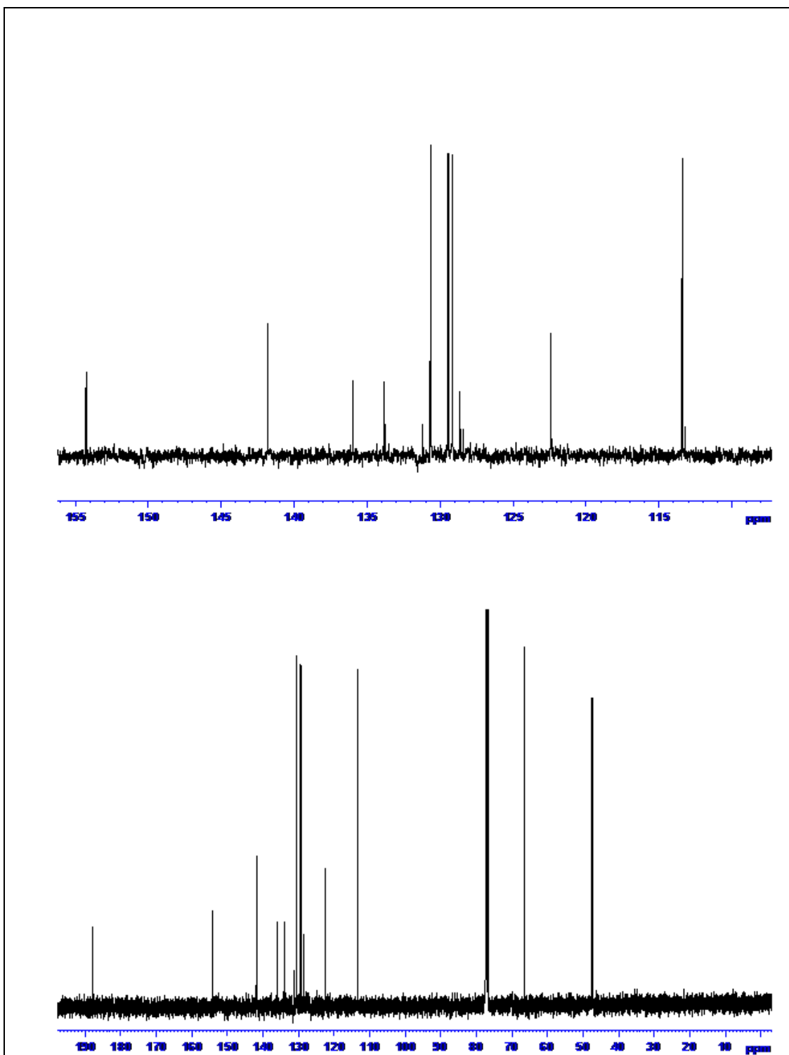
Figure 12. ^{13}\text{C} NMR spectrum of compound 4
