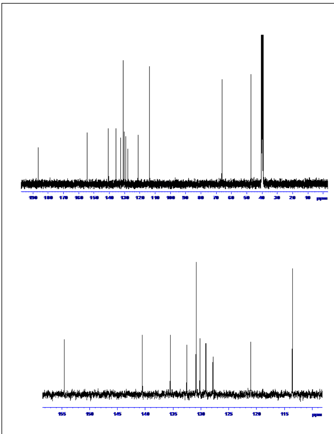
Figure 6. ^{13}\text{C} NMR spectrum of compound 2
