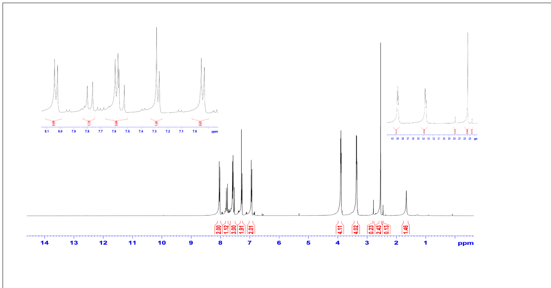
Figure 22. 1 H NMR spectrum of compound 8
