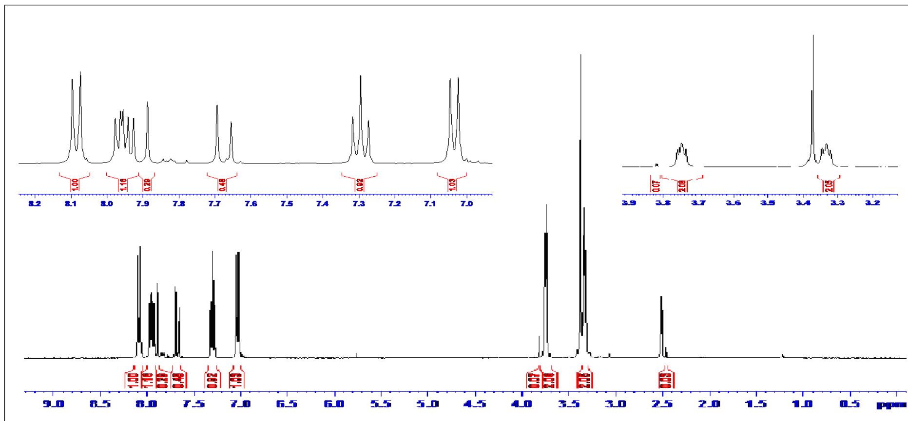
Figure 19. 1 H NMR spectrum of compound 7
