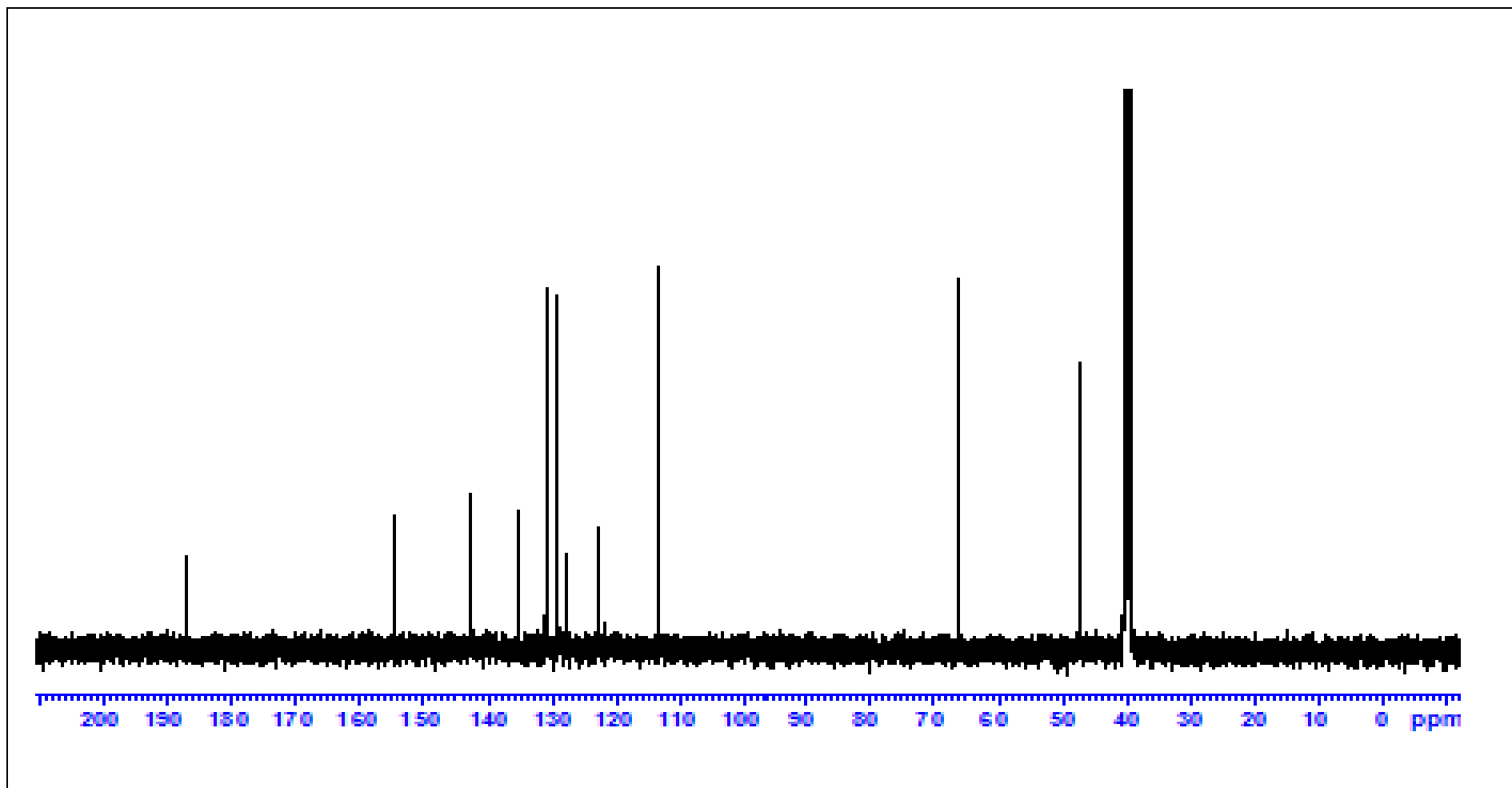
Figure 9. ^{13}\text{C} NMR spectrum of compound 3
