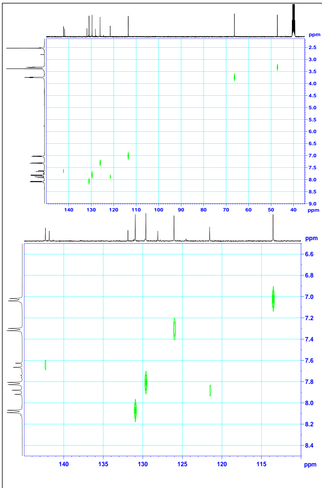
Figure 25. HETCOR NMR spectrum of compound 8
