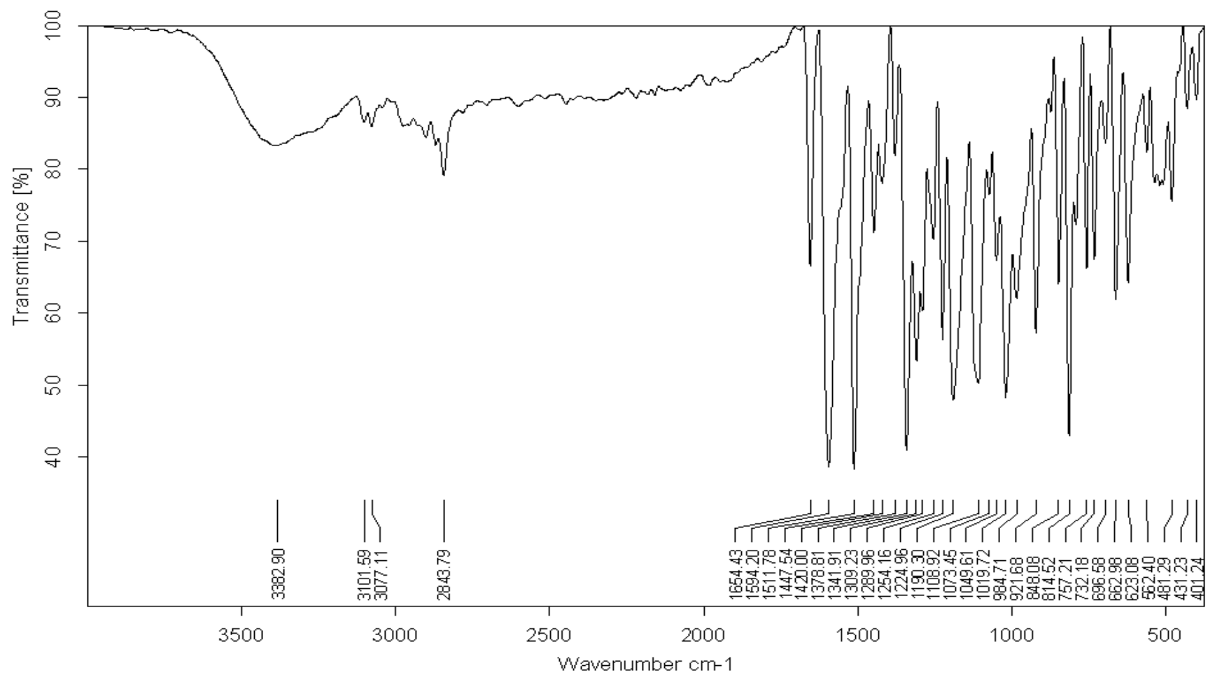
Figure 29. FT-IR spectrum of compound 10
