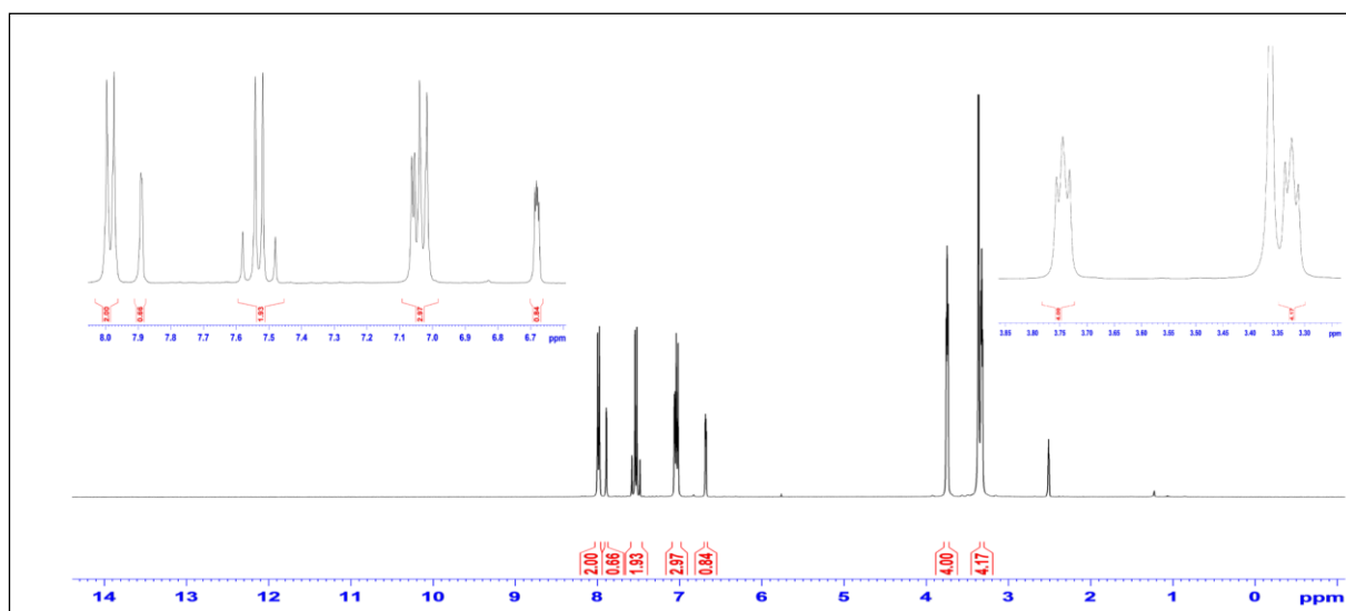
Figure 2. 1 H NMR spectrum of compound 1
