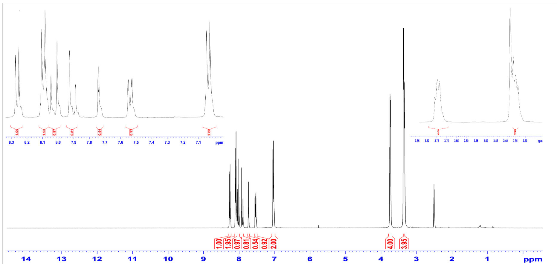
Figure 11. 1 H NMR spectrum of compound 4
