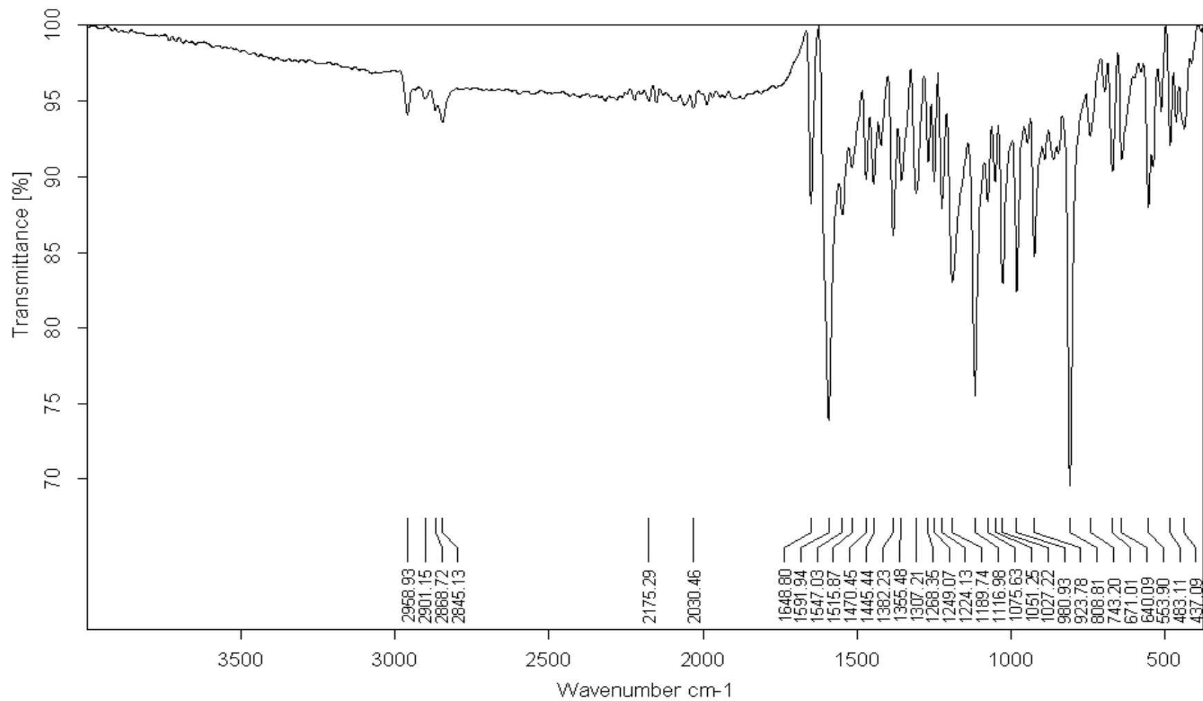
Figure 16. FT-IR spectrum of compound 6
