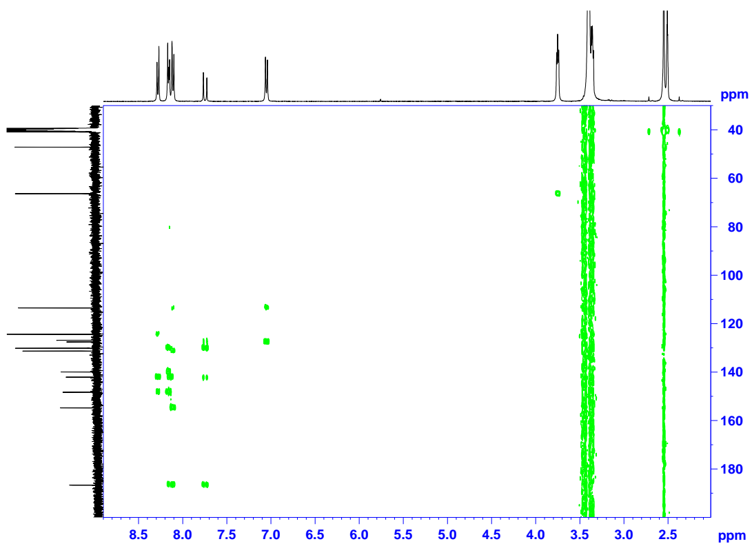
Figure 36. HMBC spectrum of compound 10
