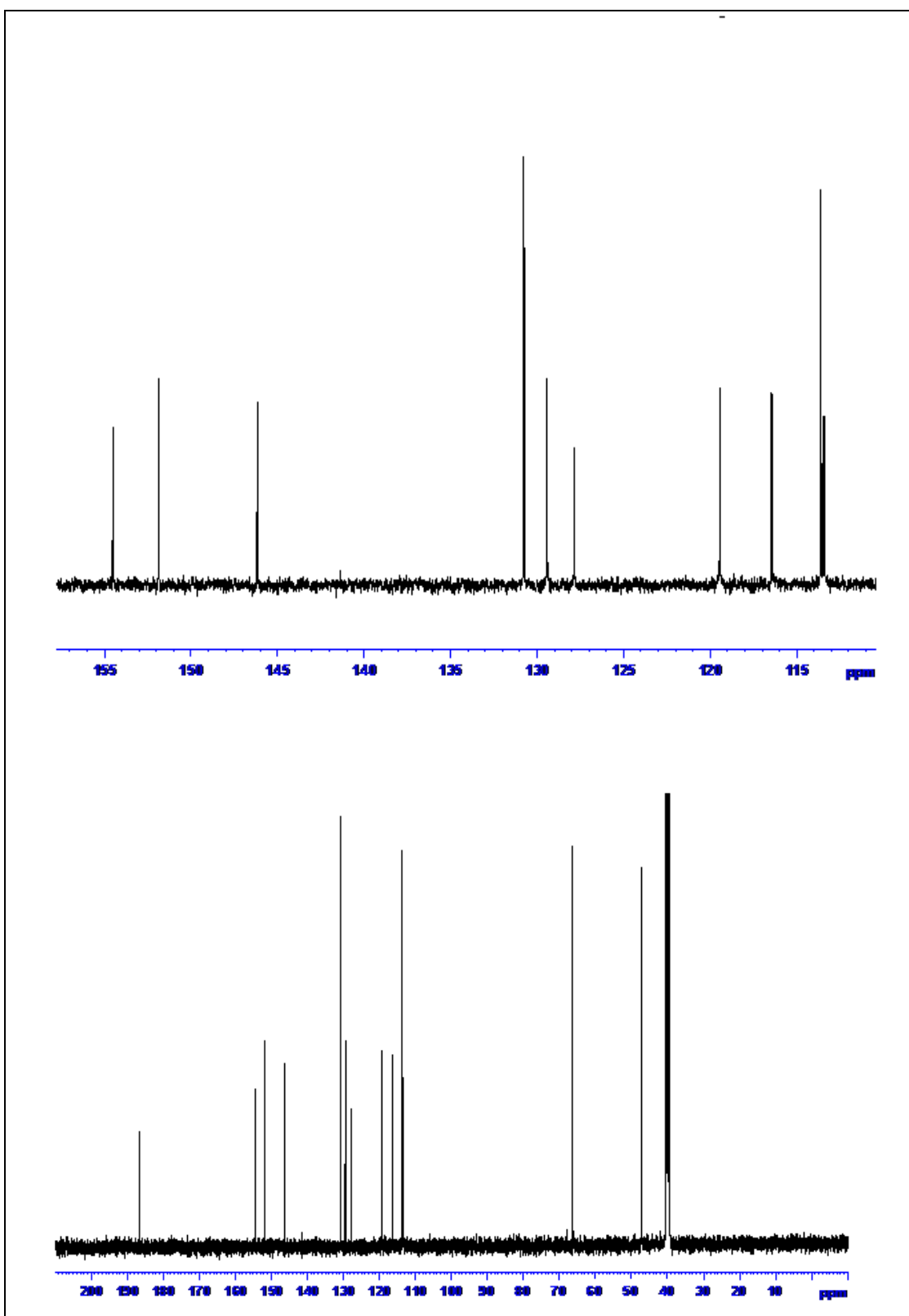
Figure 3. ^{13}\text{C} NMR spectrum of compound 1
