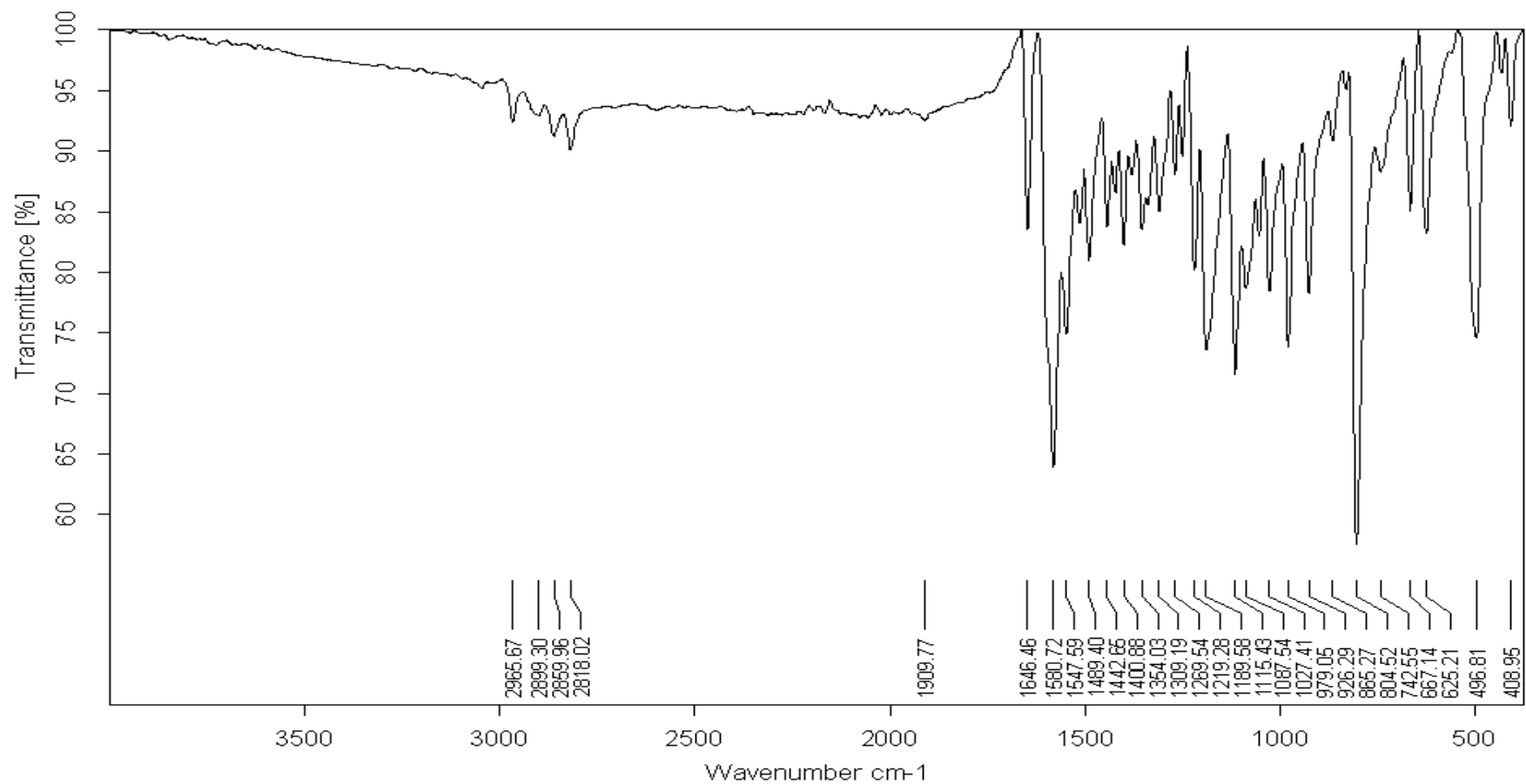
Figure 21. FT-IR spectrum of compound 8
