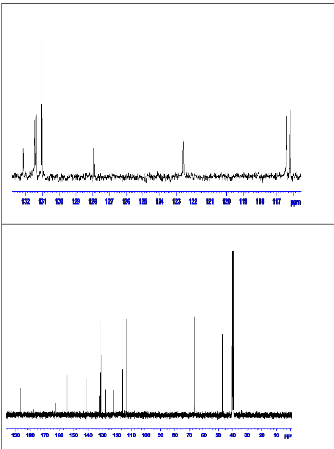
Figure 20. ^{13}\text{C} NMR spectrum of compound 7
