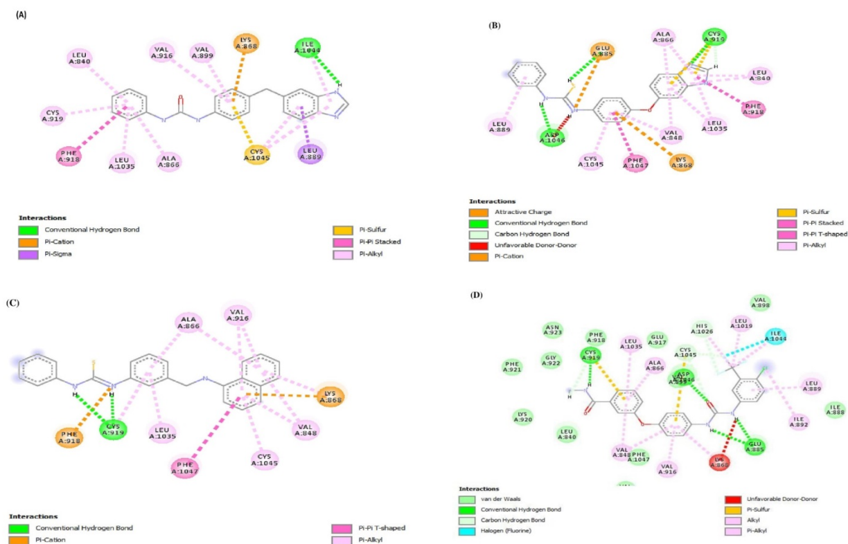
Figure 3. 2D interaction of compounds with PDB ID- 2XIR; A) Compound 1 - 2XIR B) Compound 2 - 2XIR, C) Compound 3 - 2XIR, D) Sorafenib - 2XIR
