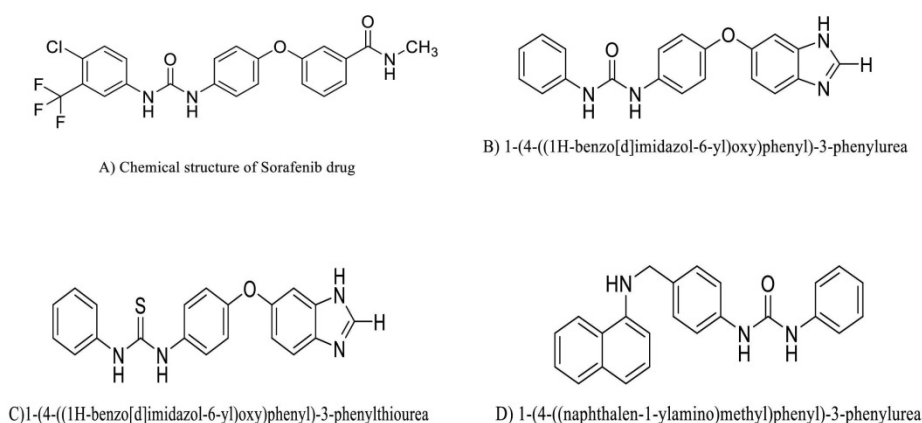
Figure 2. A) Chemical structure of Sorafenib B) Structure of compound 1 C) Structure of compound 2 D) Structure of compound 3
