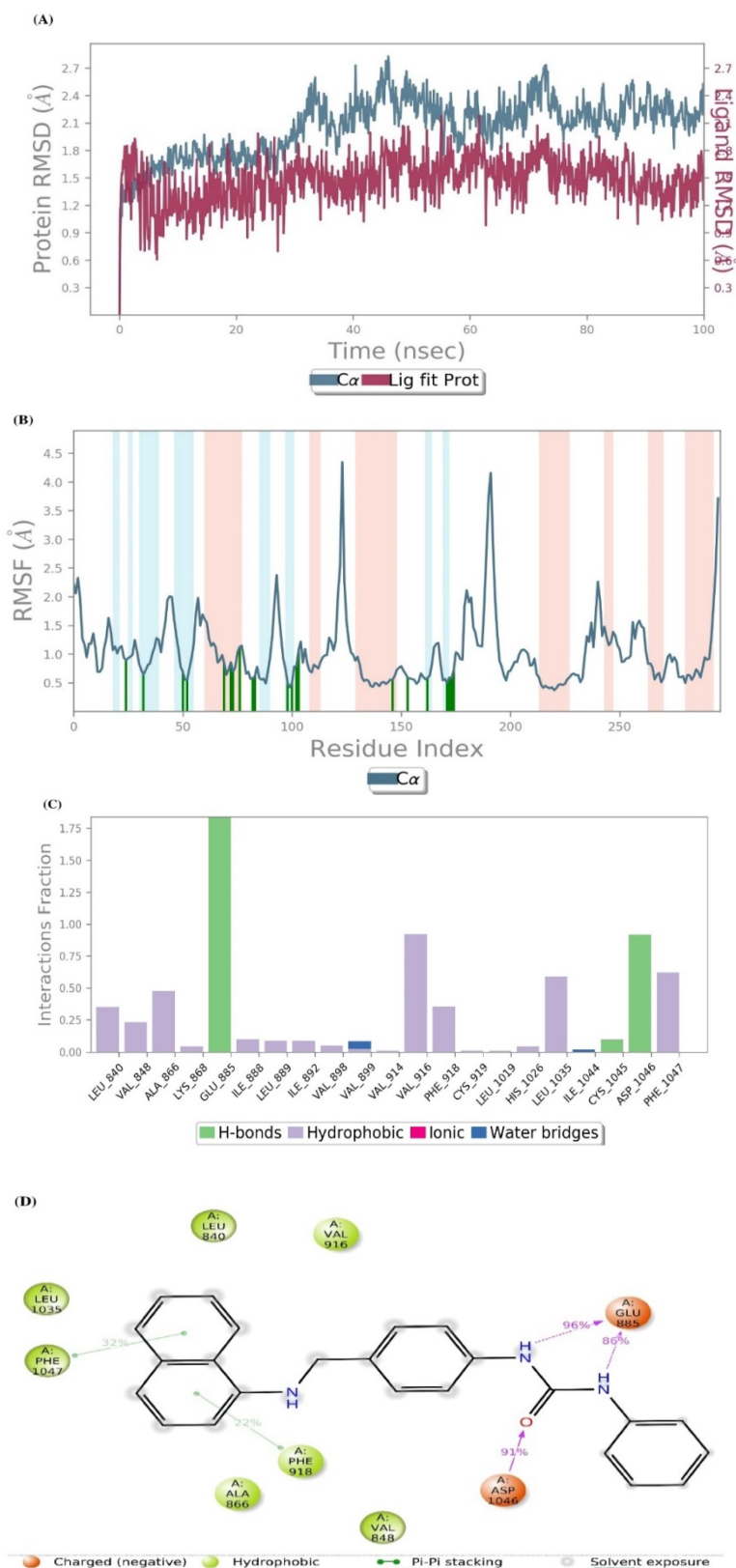
Figure 5. A) Protein and ligand RMSD values generated by a 100ns MD simulation B) Protein RMSF values generated by a 100ns MD simulation C) The protein-ligand interactions of the ligands with 2XIR during 100 ns MD. D) A 2D diagram to demonstrate protein residue-ligand atom interactions.
