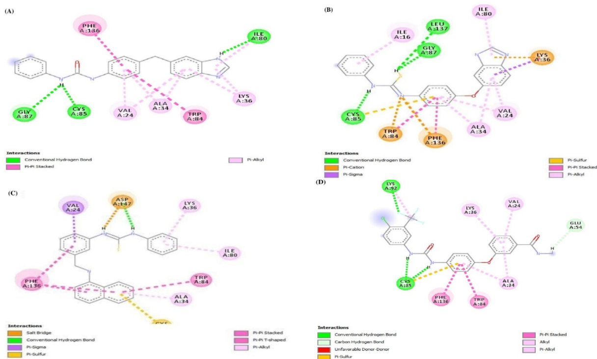
Figure 4. 2D interaction of compounds with PDB ID - 3OMV; A) Compound 1 - 3OMV B) Compound 2 - 3OMV, C) Compound 3 - 3OMV, D) Sorafenib - 3OMV
