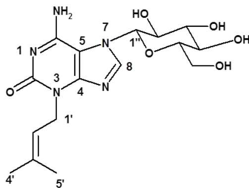
Figure 4. Locustoside A
