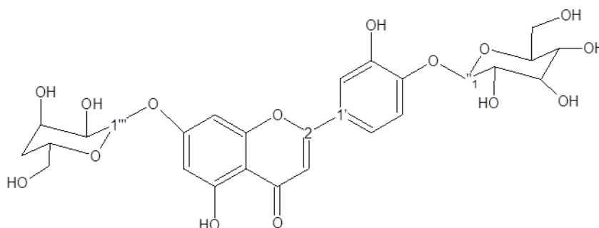
Figure 7. Luteolin-4',7-diglucoside
