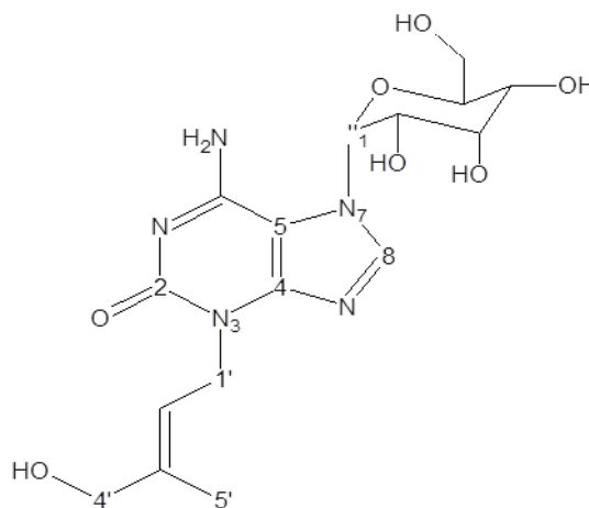
Figure 5. Saikachinoside A
