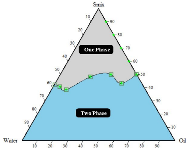
Figure 4: Pseudo ternary phase diagram for oleic oil, S_{mix} (tween 80: ethanol in 1:2 ratio) and water (Fx6-Fx10)
