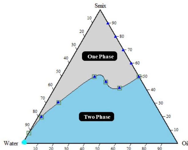
Figure 8: Pseudo ternary phase diagram for oleic oil, S_{mix} (Cremophor: Ethanol in 1:3 ratio) and water (Fx26-Fx30)
