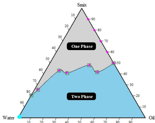
Figure 6: Pseudo ternary phase diagram for oleic oil, S_{mix} (Cremophor: Ethanol in 1:1 ratio) and water (Fx16-Fx20)
