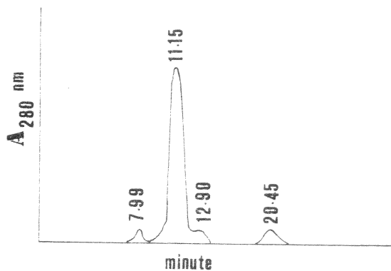
Fig. 7 : The HPLC chromatogram of prothrombin obtained from the fraction B pool after Sepharose CL-6B column chromatography (pool 1). (Sample volume: 10 \mu l, AUFS : 0.05, flow rate : 0,6 ml/min, RT 11.15: prothrombin activity; RT 20.45: Factor IX activity).
