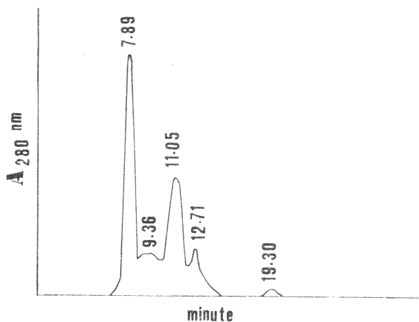
Fig. 6 : The HPLC chromatogram of the B fraction pool obtained from DEAE Sephadex A-50 column chromatography. (Sample volume : 10 \mu l, AUFS : 0.05, flow rate: 0,6 ml/min; RT 11.05 : prothrombin activity; RT 12.71: thrombin activity).
