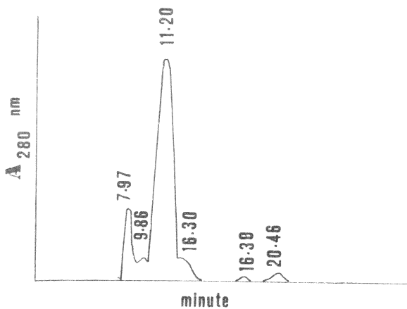
Fig. 5 : The HPLC chromatogram of prothrombin complex. (sample volume 7,5 \mu l, AUFS: 0.1, flow rate : 0,6 ml/min, RT 11.20: prothrombin activity; RT 12.93 : thrombin activity).
