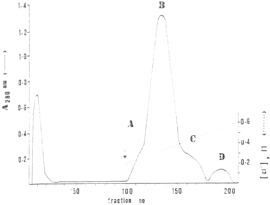
Fig. 1: DEAE Sephadex A-50 column chromatography of prothrombin complex. Column diameter 3.5 cm; height 22 cm; flow rate: 1.35 ml/min; fraction volume: 16 ml; Equilibrium buffer : 0.2 M NaCl and 1 mM benzamidin HCl containing 0.05 M \text{Na}_2\text{HPO}_4 / \text{NaH}_2\text{PO}_4 buffer, pH 6.00; linear gradient : equilibrium buffer and 0.6 M NaCl and 1 mM benzamidin HCl containing 0.05 M \text{Na}_2\text{HPO}_4 / \text{NaH}_2\text{PO}_4 buffer, pH 6,00. The arrow shows the start of the gradient; pool A : fractions 102-119; pool B = fractions 120-150; pool C = 151-180; pool D = 181-210).
