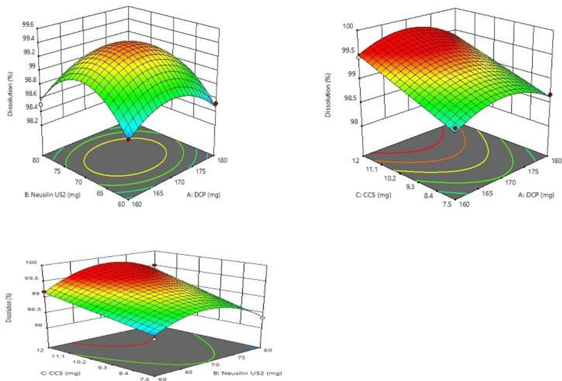
Fig. 5. 3-D Surface response graph for Dissolution
