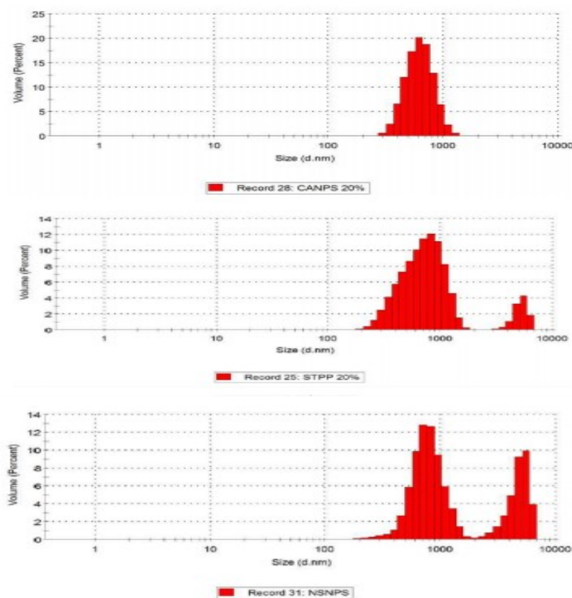
Figure 2: Particle size distribution of native and cross-linked starch nanoparticles CANP – Citric acid nanoparticles STPP – Sodium tripolyphosphate nanoparticles NSNP – Native starch nanoparticles
